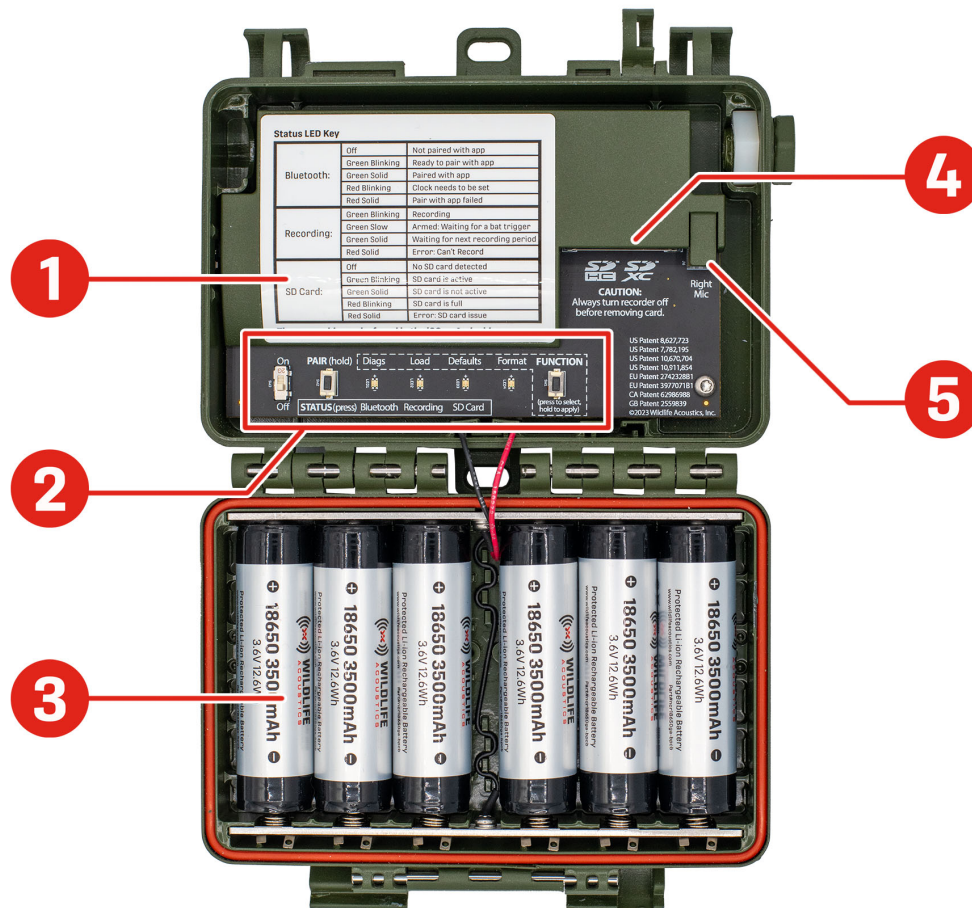
Figure 5. Internal Overview
