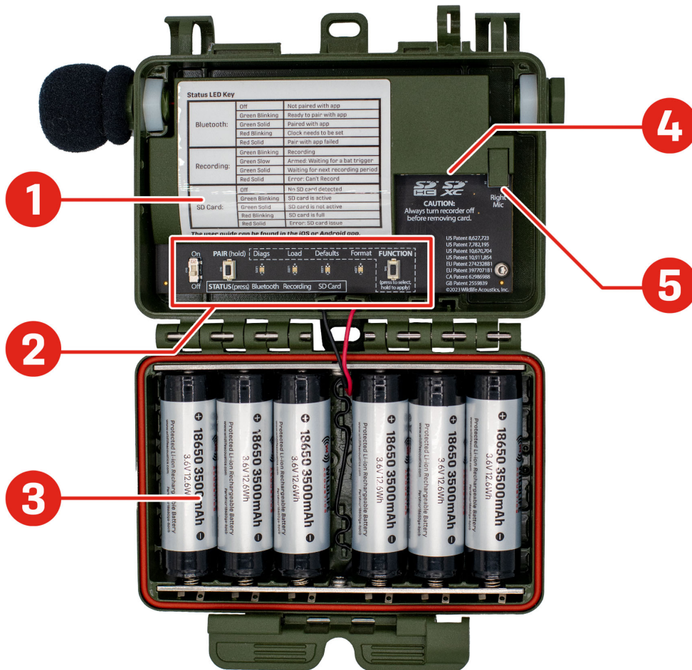
Figure 4. Internal Overview
