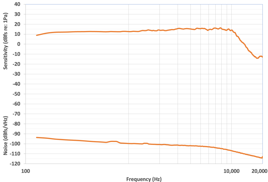
Figure 7. Sensitivity and Noise Floor, Logarithmic Frequency Scale
